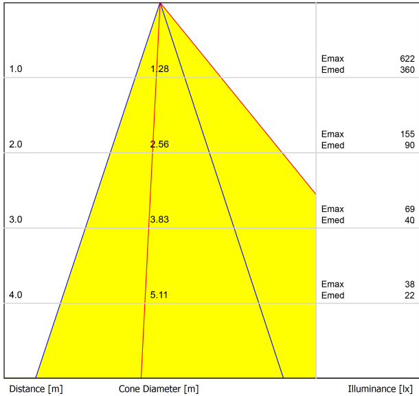
CONICAL DIAGRAM
