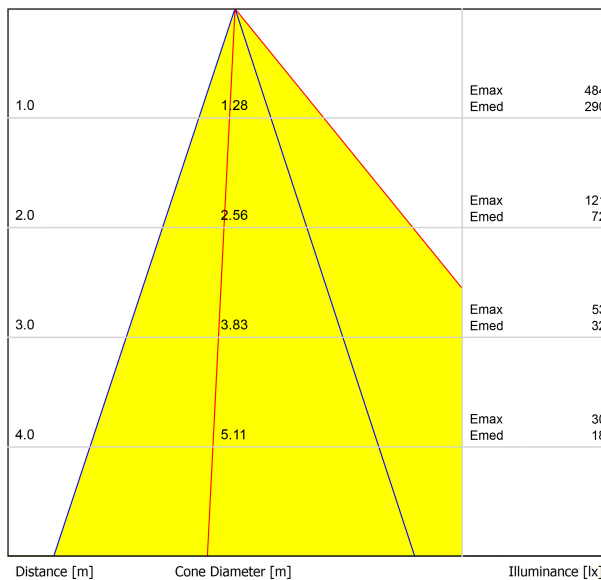
CONICAL DIAGRAM
