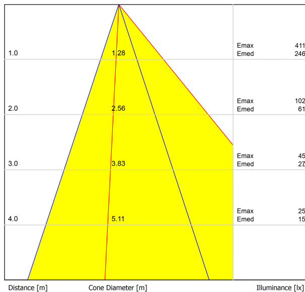
CONICAL DIAGRAM
